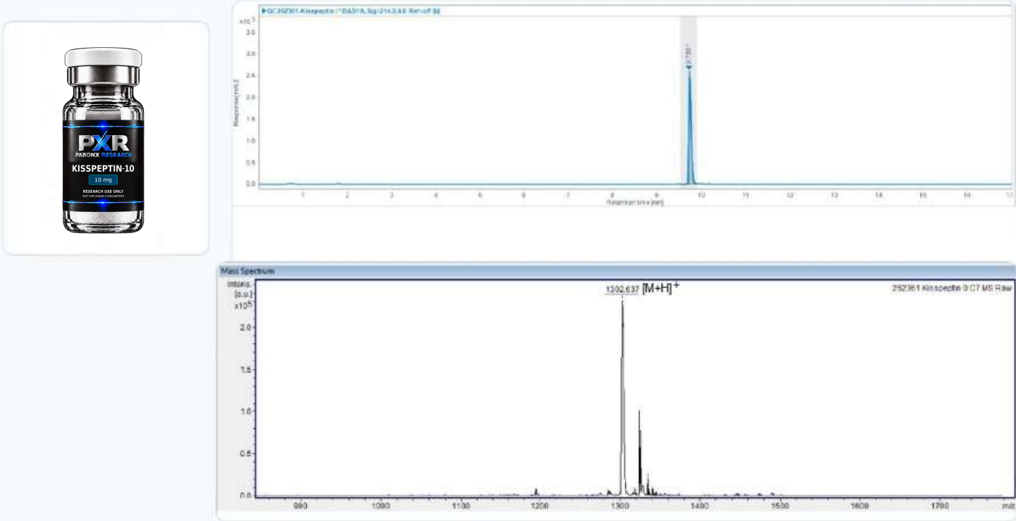
HPLC Chromatogram (Retention Time: 9.733 min)
