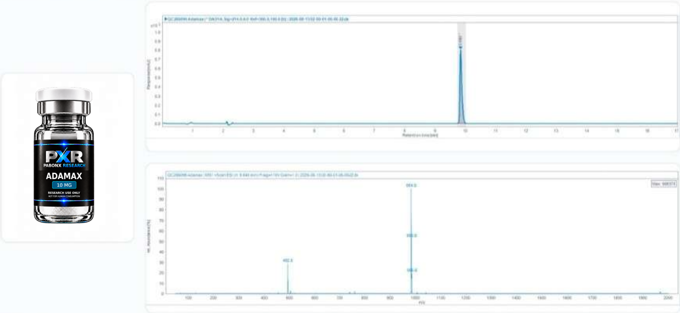
HPLC Chromatogram · Retention Time 9.840 min
